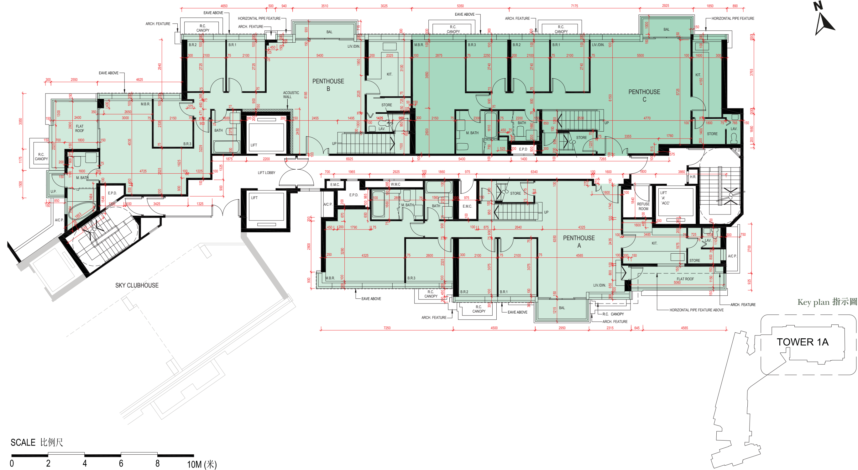
TOWER 1A 35/F PENTHOUSE FLOOR FLOOR PLAN
