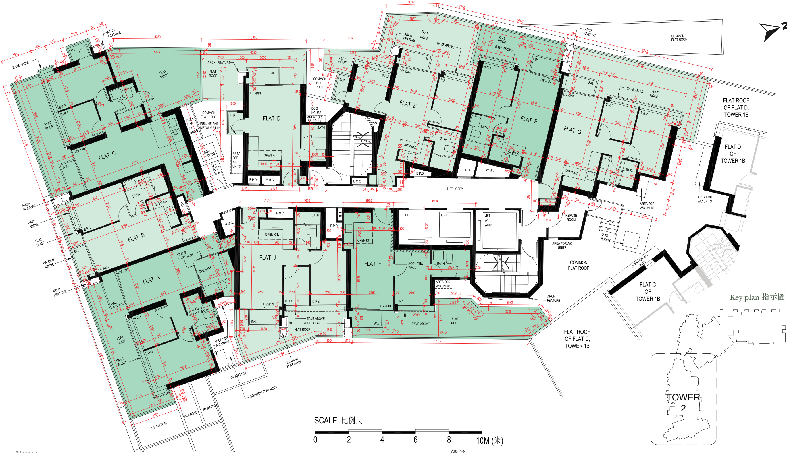
TOWER 2 3/F (GARDEN FLOOR) FLOOR PLAN
